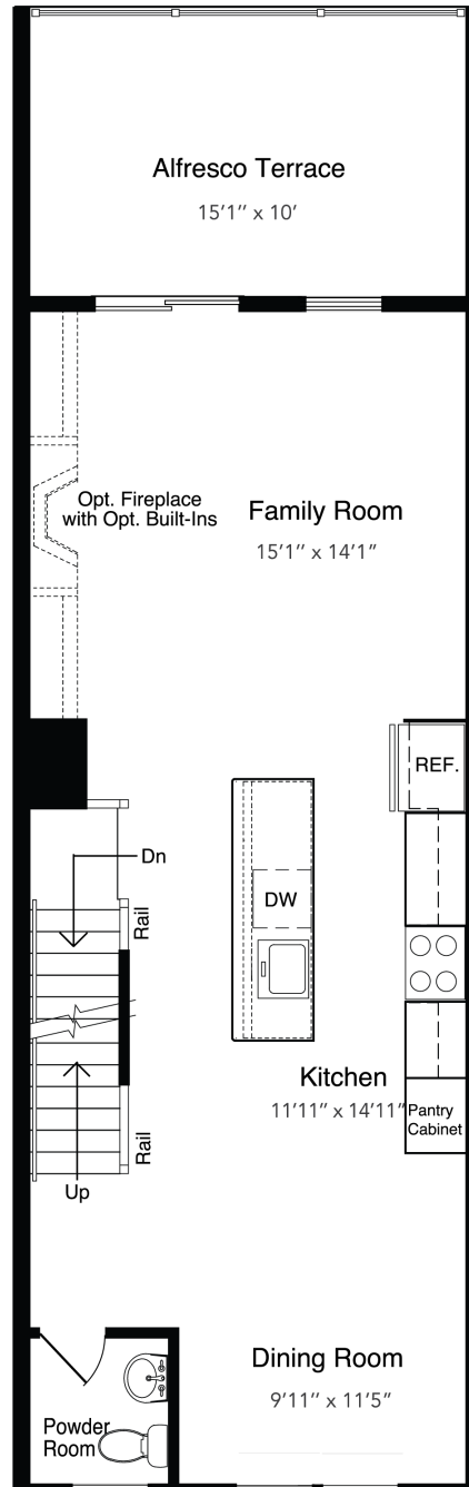
The Barrett Alternate Second Floor Plan Window Patterns Vary By Elevation
